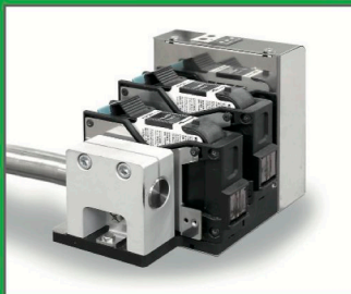
▲ Two cartridges with print height of 25 mm
