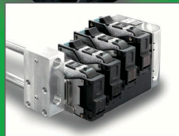
▲ Four cartridges with print height of 50 mm
