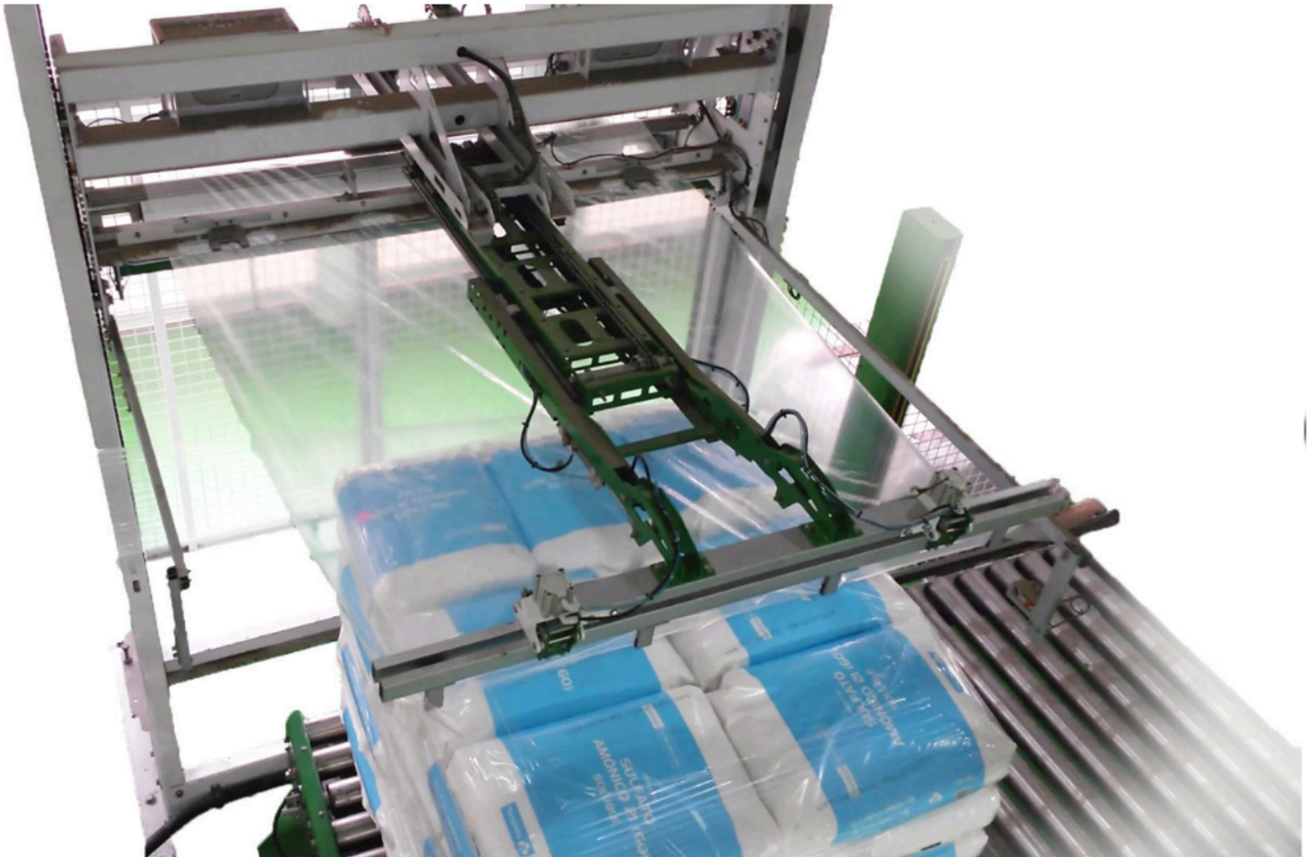
AUTOMATIC TOP PALLET COVER SYSTEM
